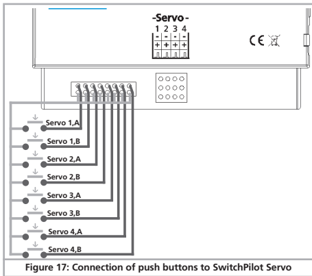
Figure 17: Connection of push buttons to SwitchPilot Servo
