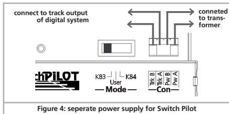
Figure 4: separate power supply for Switch Pilot
