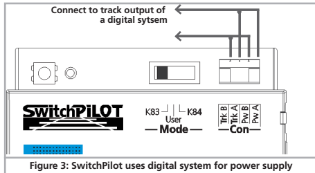
Figure 3: SwitchPilot uses digital system for power supply
